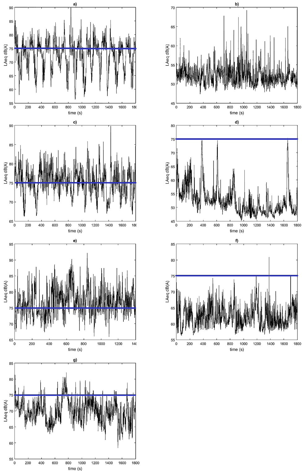
Figure 3. Time data series of the sound measurements (LAeq units in dB(A)), blue line according to allowed local noise level: a) Ciudad de Cali Avenue road, b) Industrial area, c) Cll 13 Avenue road, d) Residential area, e) Transmilenio Salitre - El Greco station, f) Commercial area Gran Estacion shopping center, and g) Commercial area Diverplaza shopping center.
